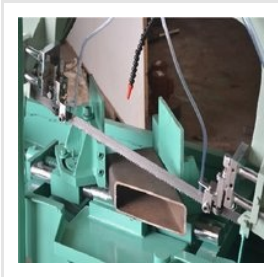
Angular Cutting Bandsaw Machine
